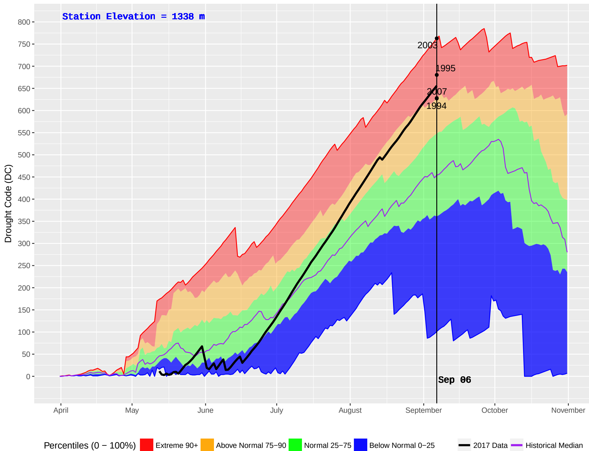
EIGHT MILE (391) : Historical (1980–2016) and Current (2017) Noon Drought Code (DC)
